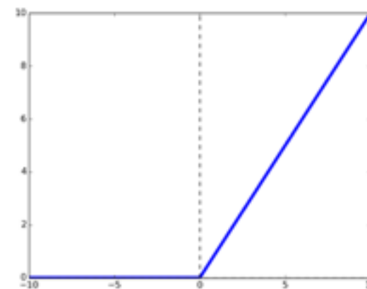
ReLU
